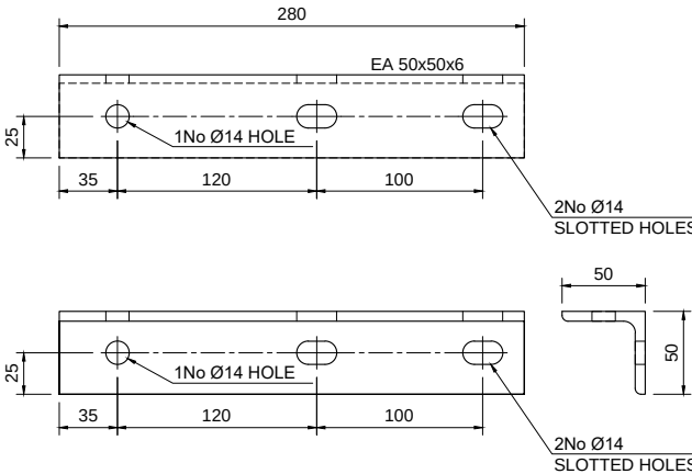
TPA-BR-2 - EA50x50x6 Scale 1:5
