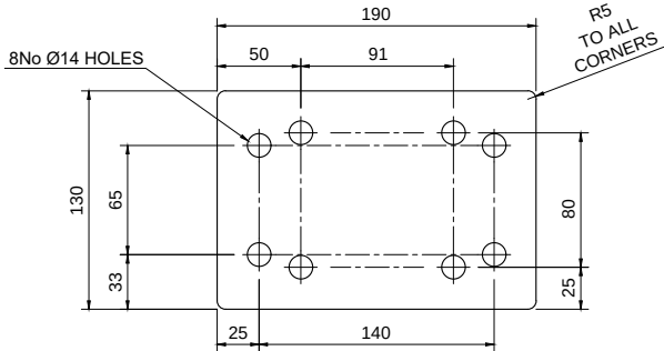
TPB-BR-3 - 10mm THICK Scale 1:5
