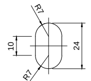
SLOTTED HOLE DETAIL Scale 1:2
