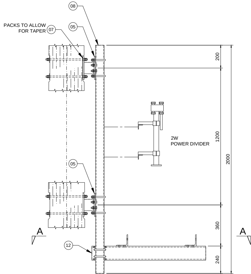
DETAIL H - Rx ANTENNA MOUNT Scale 1:20
