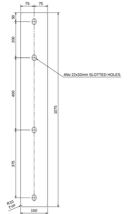
TPC-B - 15mm THICK Scale 1:10
