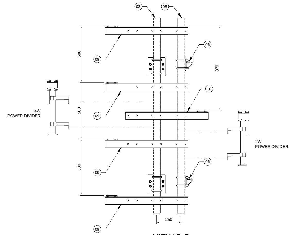
VIEW B-B Scale 1:20
