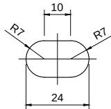
SLOTTED HOLE DETAIL Scale 1:2
