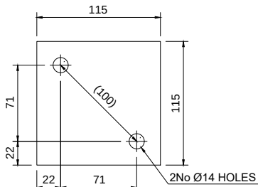
PART TPL-1 - 10mm THICK Scale 1:5
