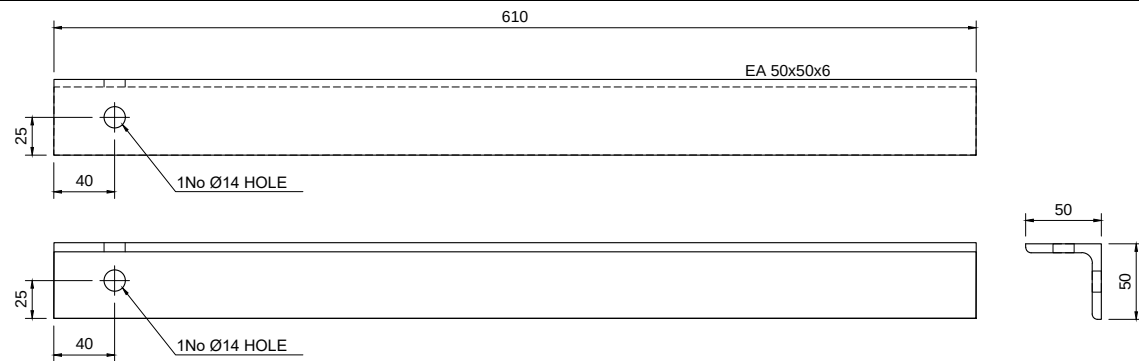
TPA-BR-1 - EA50x50x6 Scale 1:5
