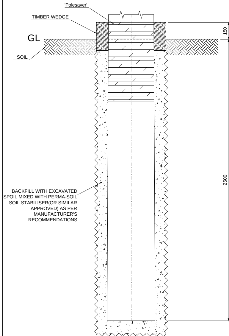
INSTALLATION ELEVATION Scale 1:20
