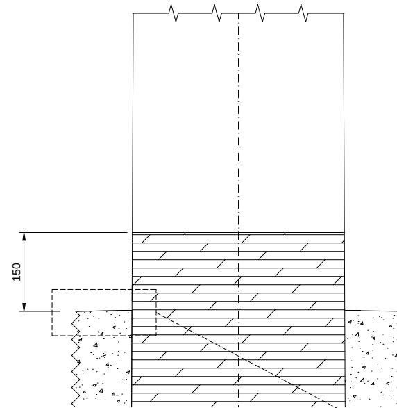
WATER PROOFING Scale 1:10
