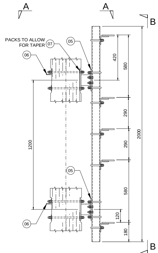
DETAIL G - Tx ANTENNA MOUNT Scale 1:20
