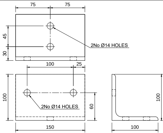
TPL-C-2 - EA100x100x8 Scale 1:5
