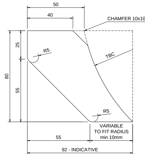
TPC-A-2 - 10mm THICK Scale 1:2
