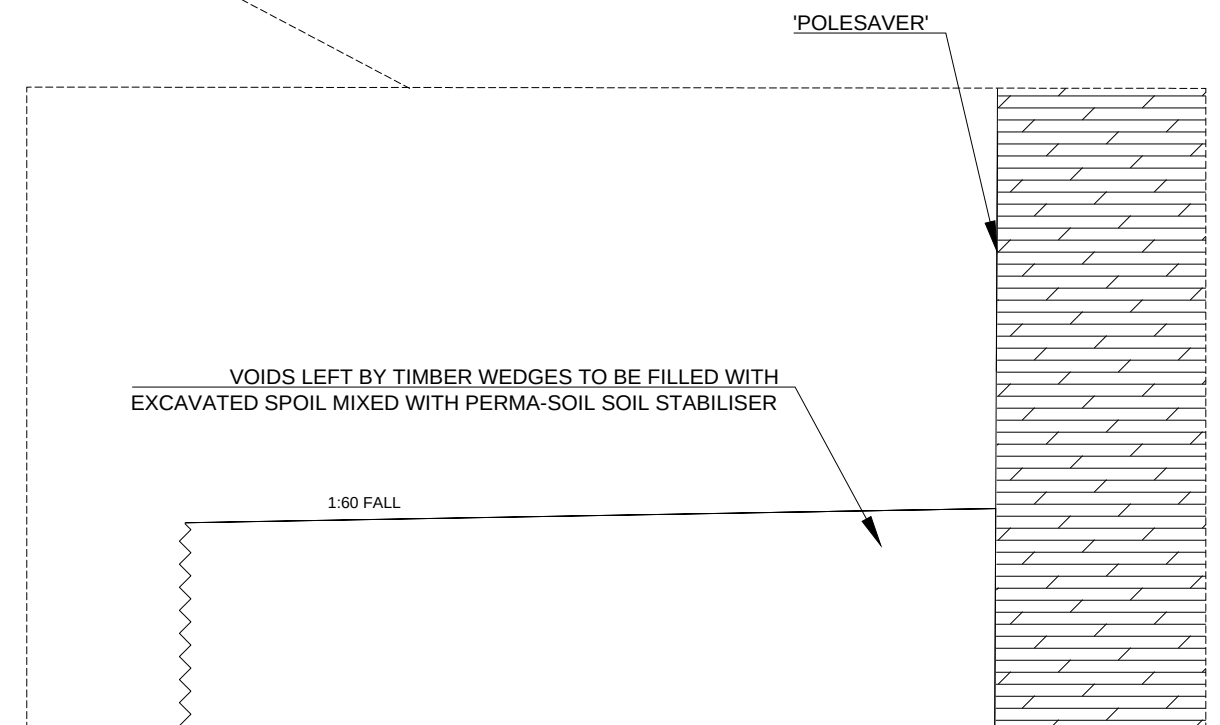
ENLARGED DETAIL Scale 1:1
