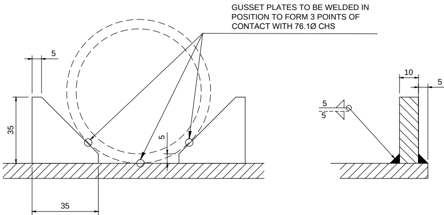
TYPICAL GUSSET PLATE DETAIL Scale 1:2
