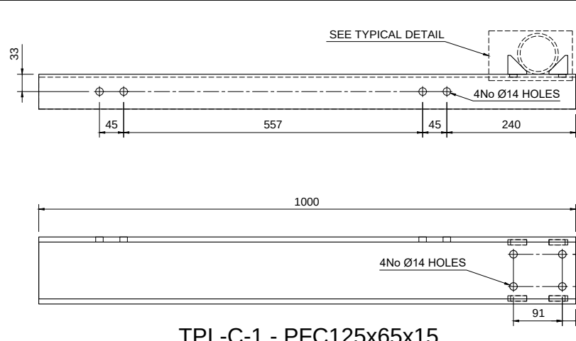
TPL-C-1 - PFC125x65x15 Scale 1:10
