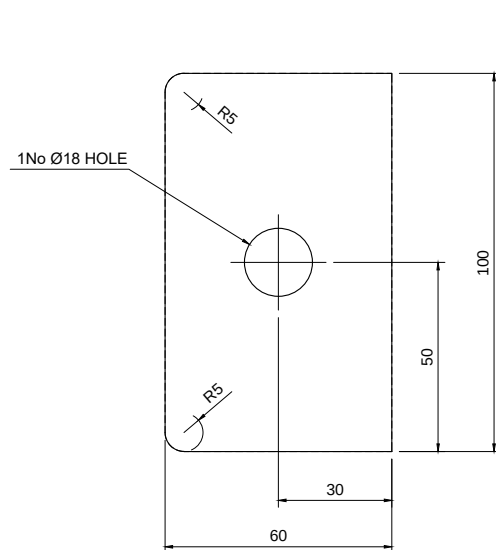
TPC-A-1 - 15mm THICK Scale 1:2
